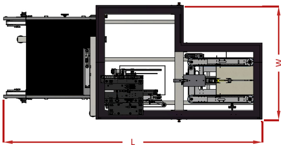
Dimensions shown in table below. Layout represents large machine. Multiple layouts and machine handing options available.
